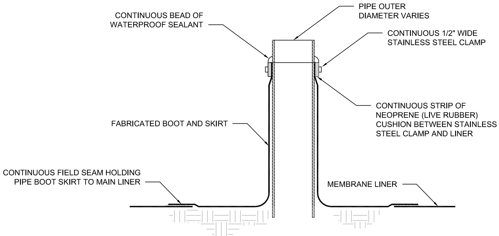
TYPICAL 90° PIPE BOOT (NTS)
