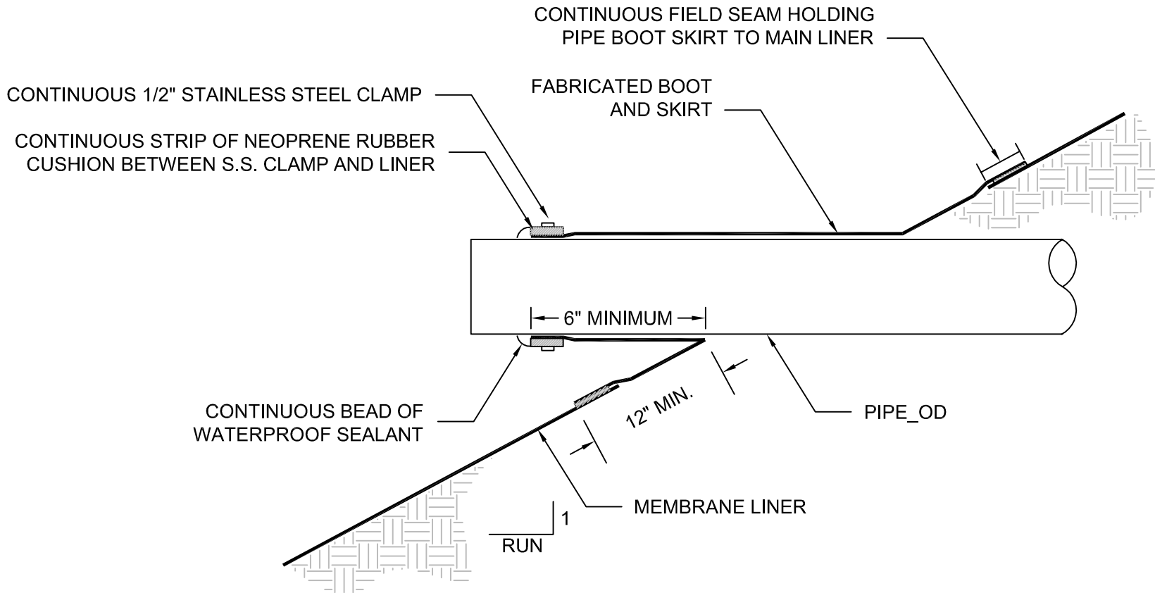
TYPICAL PIPE BOOT (NTS)
