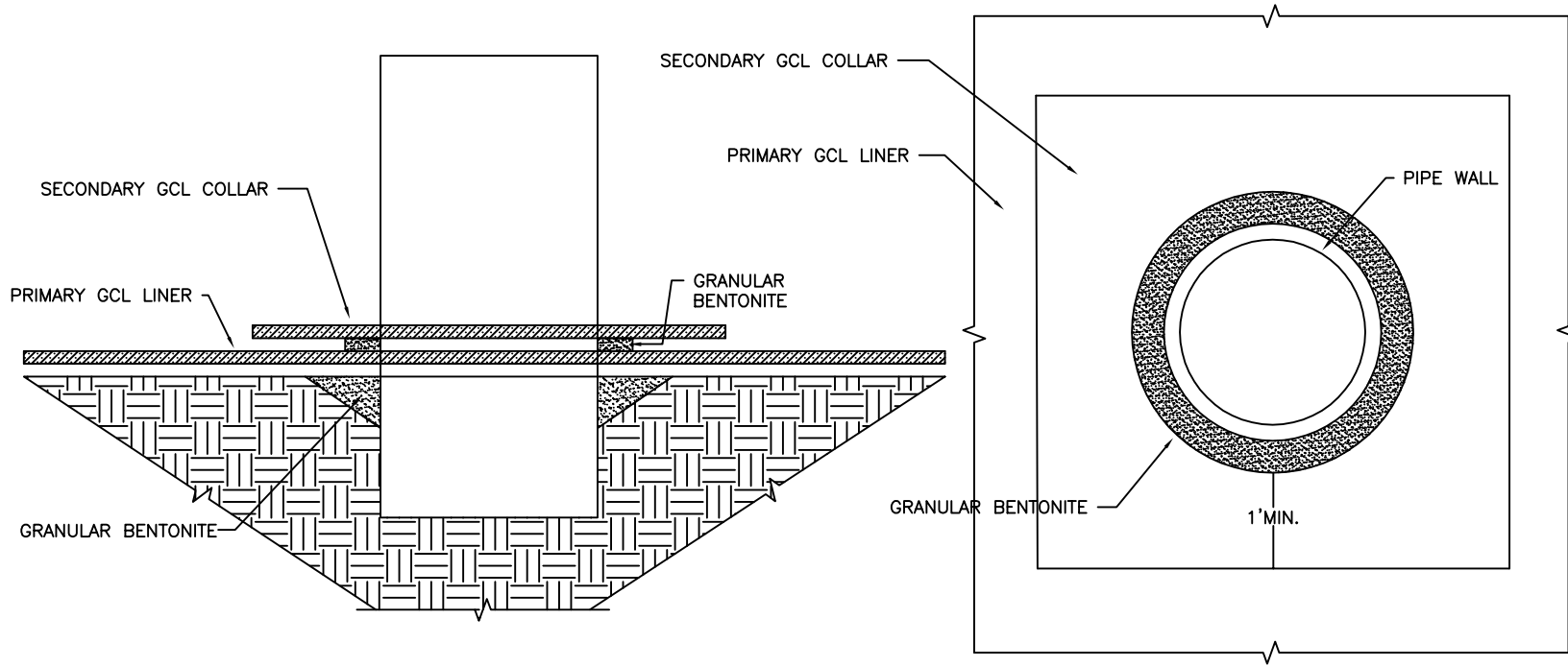
GCL PIPE PENETRATION (90 DEGREES)
