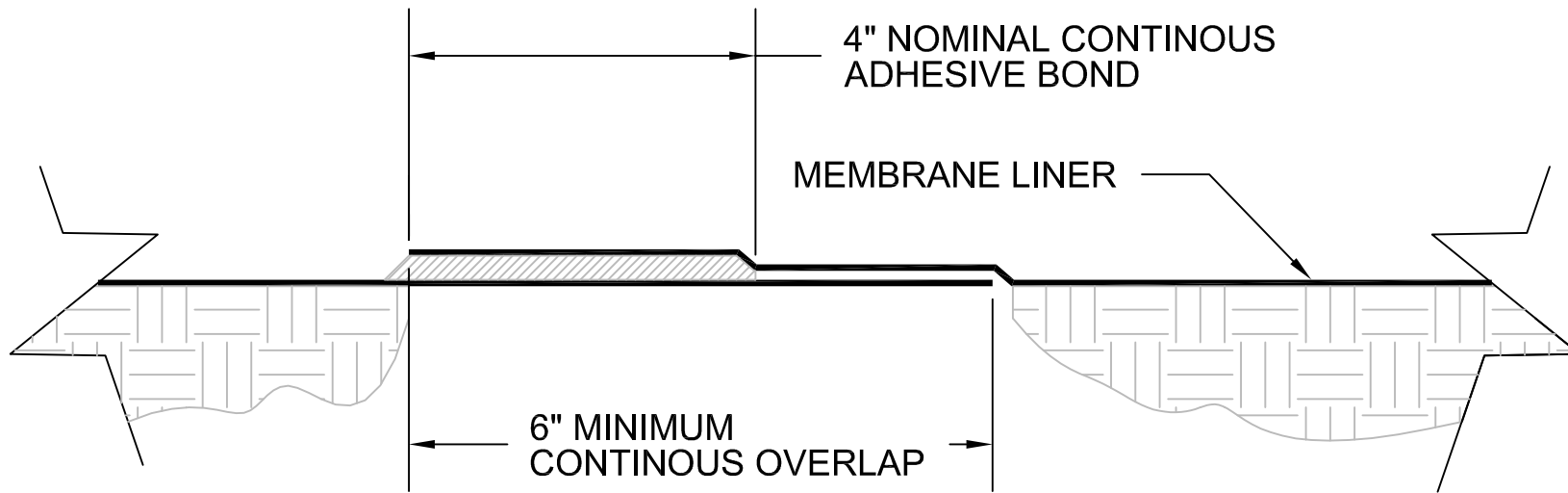
PVC ADHESIVE FIELD SEAM DETAIL (NTS)
